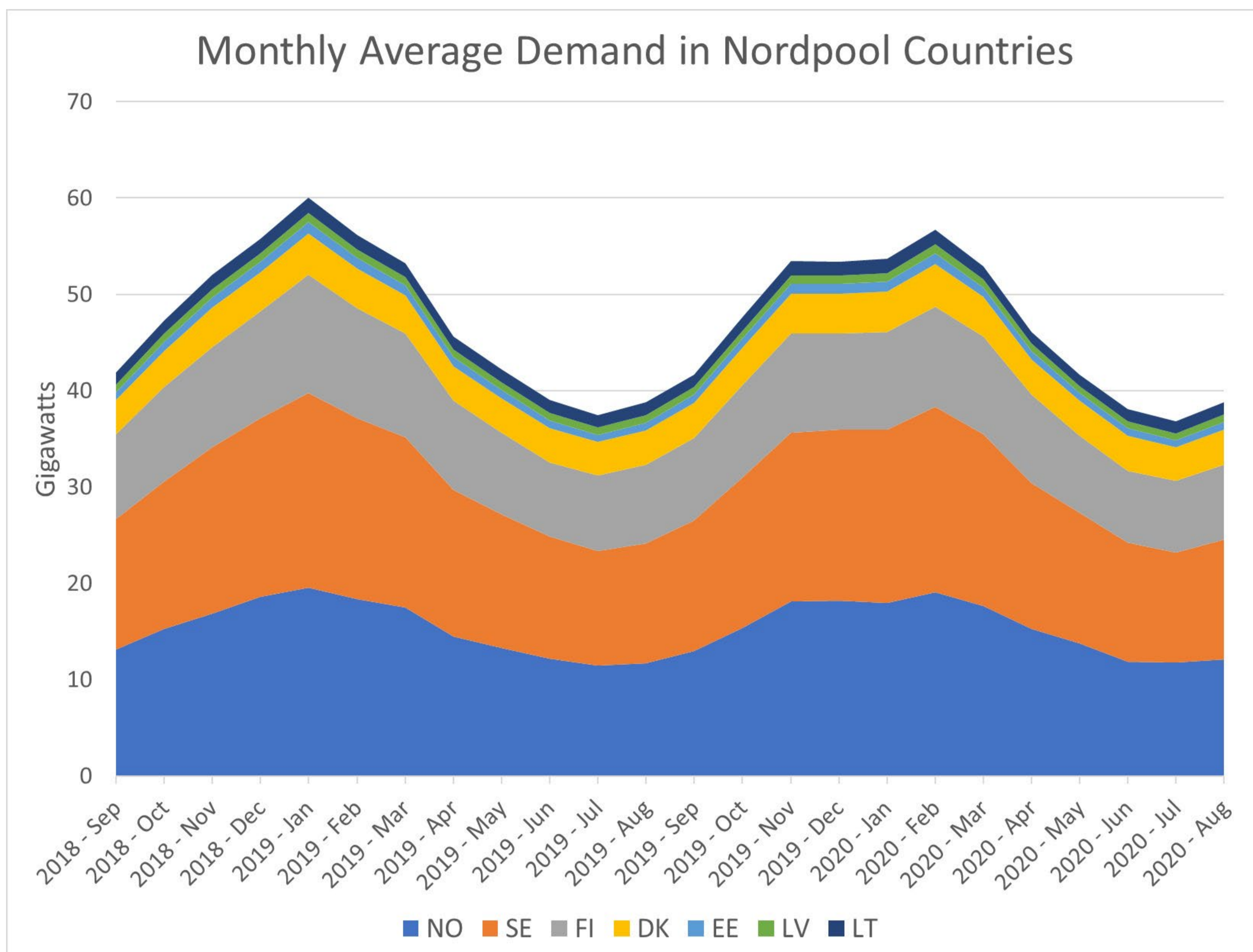
Figure 3: Monthly average demand in Nordpool countries from September 2018 to August 2020. Data: Nordpool.
